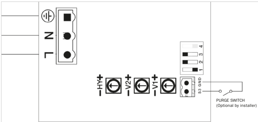
Fig.1 Control box
