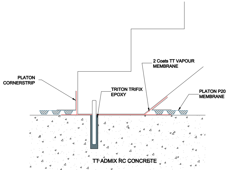
1. Waterproofing Detail Precast Stair To Floor
