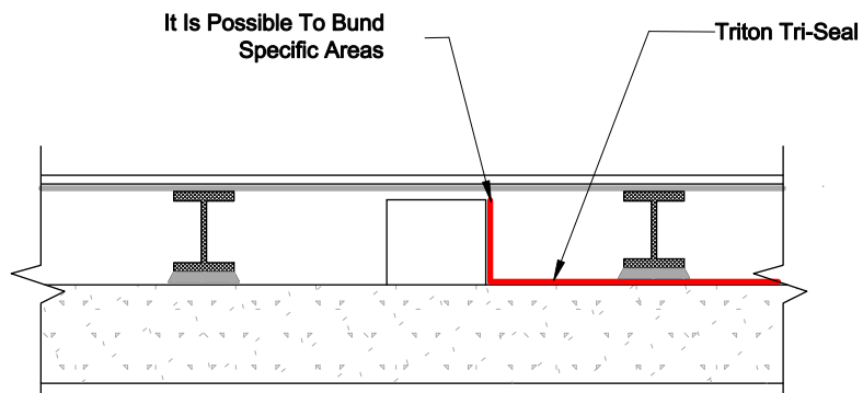
RAISED ACCESS FLOOR - BUNDED AREA
