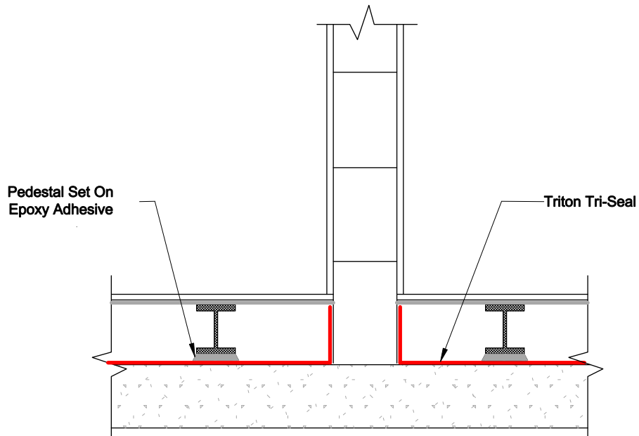
RAISED ACCESS FLOOR - INTERNAL WALL
