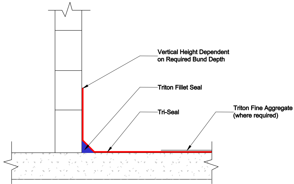
PLANT ROOM BUNDED AREA
