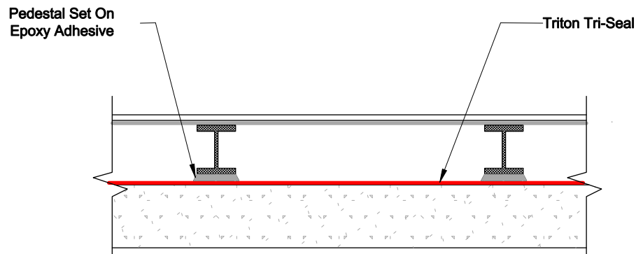
RAISED ACCESS FLOOR
